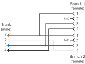
S15YA4-M124-M124-0.2M Non-parallel 4-Pin Wiring
